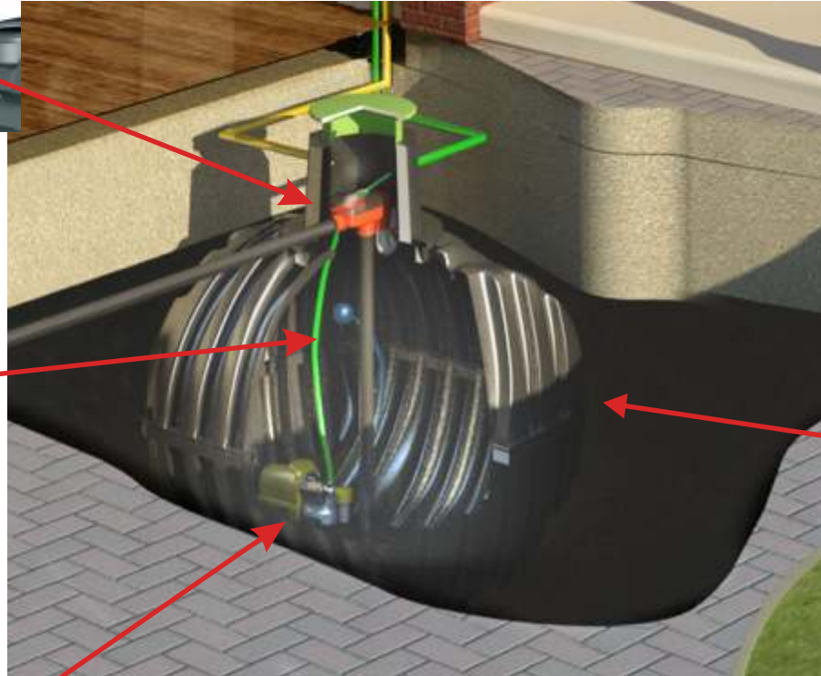
Graf Carat tank turret with Optimax Filter
