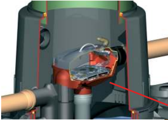
Graf Carat tank turret with Optimax Filter
