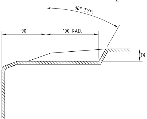
SIDE ELEVATION
